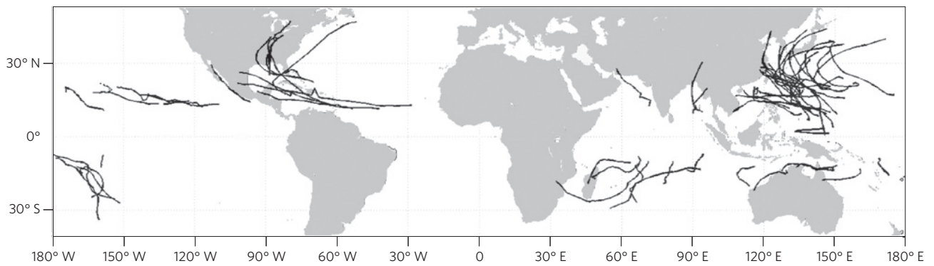
Figure 1 | Global distribution and paths of the 58 hurricanes used in this study. The category-4 and category-5 hurricanes included in this study are: 2005—Adeline, Bertie, Dennis, Emily, Haitang, Ingrid, Katrina, Kenneth, Khanun, Kirogi, Longwang, Mawar, Meena, Nabi, Nancy, Nesat, Olaf, Percy, Rita, Sonca, Talim, Wilma; 2006—Bondo, Carina, Chanchu, Chebi, Cimaron, Daniel, Durian, Ewiniar, Floyd, Glenda, Ioke, John, Larry, Mala, Monica, Saomai, Shanshan, Xangsane, Xavier, Yagi; 2007—Dean, Dora, Favio, Felix, Flossie, Gonu, Indlala, Kajiki, Krosa, Man-yi, Nari, Sepat, Sidr, Usagi, Wipha and Yutu.
