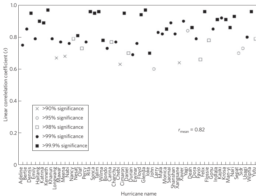
Figure 4 | The correlation coefficients ( r ) between maximum sustained winds and lightning activity. Each point represents one hurricane, and the symbols represent the level of statistical significance for a specific hurricane.
