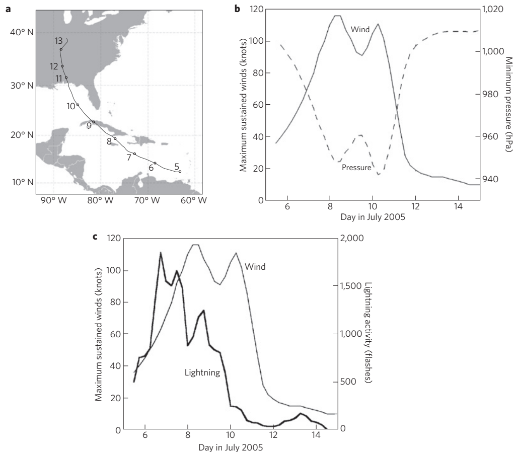
Figure 2 | Hurricane Dennis 5-14 July 2005. a , The path of Hurricane Dennis in the Atlantic Ocean, showing the location at 12:00 UTC every day. b , The minimum pressure at the centre of the hurricane (dashed curve) together with the maximum sustained winds (solid curve). c , The maximum sustained winds (solid thin curve) and the observed lightning frequencies within a 10^\circ \times 10^\circ gridbox centred on the eye of the storm.
