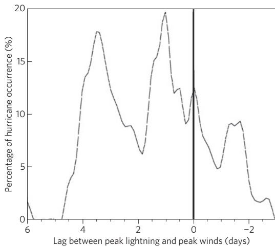
Figure 3 | Lag times between the maximum lightning activity and the maximum sustained winds in 56 hurricanes. Positive lags imply that the lightning activity peaked before the maximum intensity of the winds, and vice versa for negative lags.
